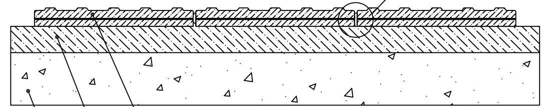
C-C (1:7)
